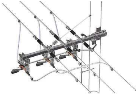
3-WIRE ALLEY ARM
