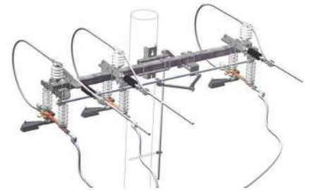
3-WIRE DEADEND RISER
